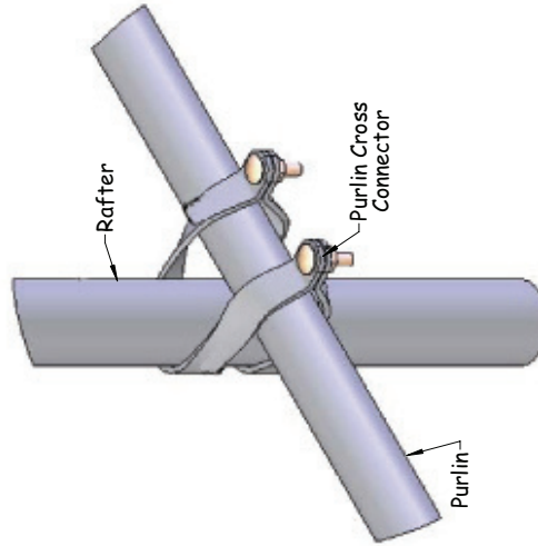
View 3 Purlin-Mid Rafter
