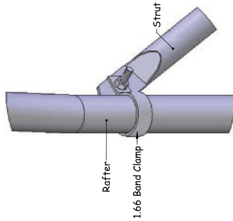
View 2 Strut Connection
